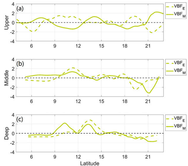
FIG. 6. (a)–(c) Zonal- and layer-integrated VBF_E (dashed lines) and VBF_M (solid lines) as a function of latitude in the upper, middle, and deep layers, respectively. The mean values were removed then normalized by the standard deviation to make the two variables comparable.
