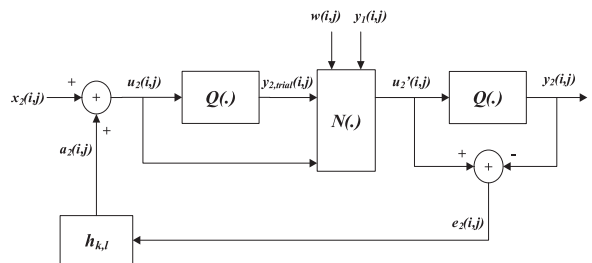
Fig. 2. DHCED system.
